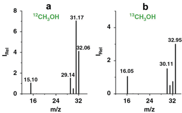
Fig. 15 GC/MS spectra and fragmentation pattern for the electrocatalyzed \text{CO}_2 conversion into \text{CH}_3\text{OH} . Graphs show the mass fragmentation pattern of \text{CH}_3\text{OH} ( m/z 29 to 33) produced employing (a) ^{12}\text{CO}_2 or (b) ^{13}\text{CO}_2 as a reactant substrate. Reproduced with permission from ref. 250.
