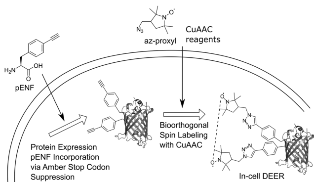
Fig. 1 Schematic overview of the in vivo spin labeling approach via copper-catalyzed [3+2] azide–alkyne cycloaddition followed by in-cell EPR distance determination. The nCAAs pENF is incorporated site-specifically into eGFP using amber stop codon suppression. The eGFP-expressing E. coli cells are subjected to CuAAC-based spin labeling and subsequent, DEER distance determination is performed directly inside the cell.
