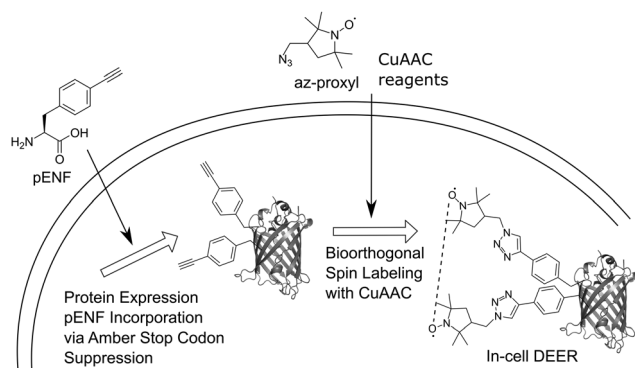
Fig. 1 Schematic overview of the in vivo spin labeling approach via copper-catalyzed [3+2] azide–alkyne cycloaddition followed by in-cell EPR distance determination. The nCAAs pENF are incorporated site-specifically into eGFP using amber stop codon suppression. The eGFP-expressing E. coli cells are subjected to CuAAC-based spin labeling and subsequent, DEER distance determination is performed directly inside the cell.
