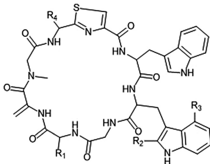
Argyirin A (30): R_1 = \text{CH}_3 , R_2 = \text{H} Argyirin C (32): R_1 = \text{CH}_3 , R_2 = \text{CH}_3 R_3 = \text{OCH}_3 , R_4 = \text{CH}_3 R_3 = \text{OCH}_3 , R_4 = \text{CH}_3 Argyirin B (31): R_1 = \text{CH}_2\text{CH}_3 , R_2 = \text{H} Argyirin D (33): R_1 = \text{CH}_2\text{CH}_3 , R_2 = \text{CH}_3 R_3 = \text{OCH}_3 , R_4 = \text{CH}_3 R_3 = \text{OCH}_3 , R_4 = \text{CH}_3 Argyirin F (34): R_1 = \text{CH}_3 , R_2 = \text{H} R_3 = \text{OCH}_3 , R_4 = \text{CH}_2\text{OH}
