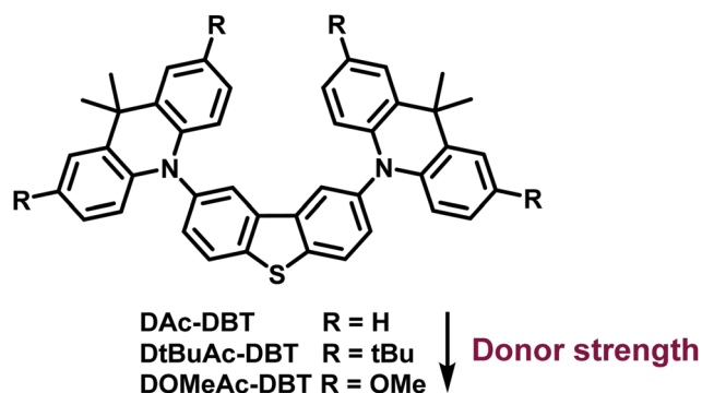
Fig. 1 Chemical structures of the DAC-DBT derivatives.
