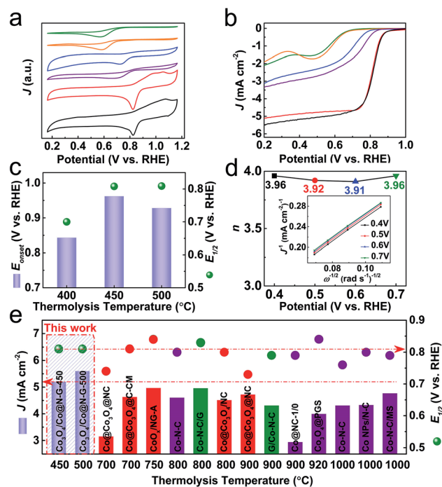
Fig. 4 ORR activity characteristics and comparative data of the samples in \text{O}_2 -saturated 0.1 M KOH: (a) CV curves (at 10 mV s -1 ) and (b) LSV curves (at 10 mV s -1 and 1600 rpm): ZDC-450 (olive), ZDC-450-A (orange), EGO-450 (blue), ZIF-67@EGO-400 (purple), \text{Co}_3\text{O}_4/\text{Co}@N\text{-G} -450 (red) and \text{Co}_3\text{O}_4/\text{Co}@N\text{-G} -500 (black). (c) Comparison of E_{\text{onset}} and E_{1/2} values against the thermolysis temperature. (d) Electron transfer number ( n ) of \text{Co}_3\text{O}_4/\text{Co}@N\text{-G} -450 as a function of potential (inset: K–L plots at different potentials calculated from Fig. S16†). (e) Comparative ORR activity data: J and E_{1/2} values against the thermolysis temperature for the catalysts in this work and other ZIF-derivatives, produced at elevated temperatures, taken from the literature (samples with second heat treatment and/or oxidation, and further acid washing are represented by red and olive colours, respectively). 21,22,24,26,30,32,33,35–37,40,48 See Table S2 in the ESI† for further details.
