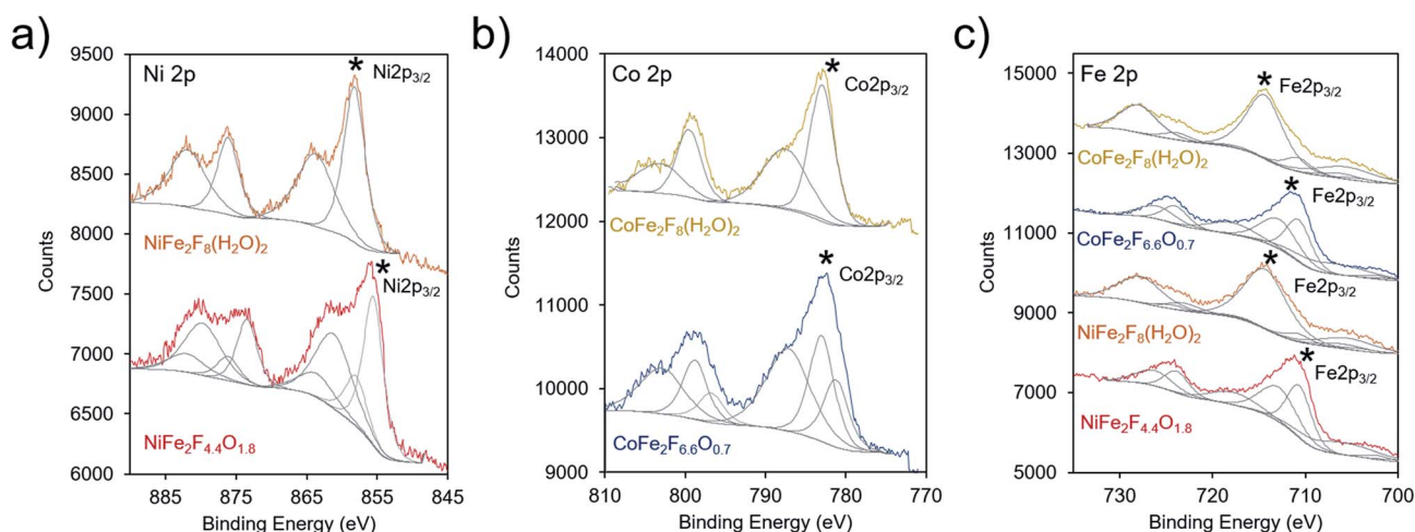
Fig. 5 XPS spectra of the (oxy)fluorides and oxyfluorides. The (a) \text{Ni } 2p_{3/2} , (b) \text{Co } 2p_{3/2} and (c) \text{Fe } 2p_{3/2} were acquired and spectra subsequently fit to (grey traces) compare with database data of F-free oxides. The 2p_{3/2} peaks discussed are denoted with a *.
