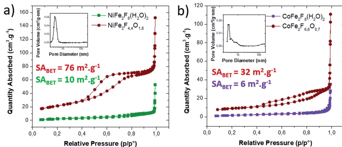
Fig. 4 \text{N}_2 adsorption/desorption isotherm of (a) \text{NiFe}_2\text{F}_{4.4}\text{O}_{1.8} and (b) \text{CoFe}_2\text{F}_{6.6}\text{O}_{0.7} before (green/purple) and after calcination (brown). Inset: corresponding BJH pore size distribution analyzed from the desorption branch.
