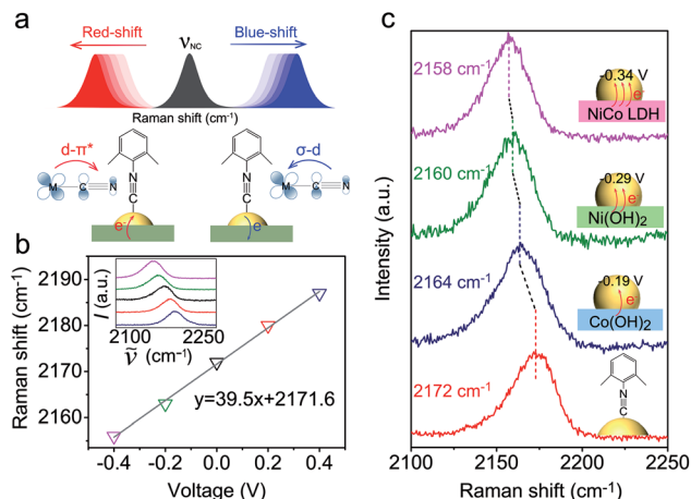
Fig. 2 SERS detection of interfacial charge transfer between Au NPs and semiconductors. (a) Schematic illustration of the interfacial charge transfer in the semiconductor–metal–molecule (DMPIC) system and the corresponding SERS band shift. (b) Raman shift of the symmetric stretching mode of \text{N}\equiv\text{C} as a function of applied voltage. The inset is the original SERS spectra showing the corresponding bands. (c) SERS spectra of DMPIC (from the bottom to the top) enhanced by Au NPs in colloidal suspension, Au/Co(OH) 2 , Au/Ni(OH) 2 , and Au/NiCo LDH, respectively.
