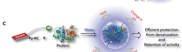
Scheme 1 Chemical structures, aggregation pattern and enzyme encapsulation. (A) Chemical structures of peptides used in this study. (B) Pictorial presentation of hydrogelation of PyKC in water through dimerization and the insolubility of the formed hydrogel in water. (C) Schematic representation of the encapsulation of proteins and prevention from denaturation in the presence of various denaturing agents.
