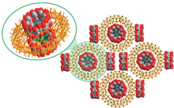
Fig. 12 Packing in the solid-state structure of \text{Na}_{15}\text{K}_3\text{H}_2\text{-}[\text{Mo}_{154}\text{O}_{462}\text{H}_{14}(\text{H}_2\text{O})_{70}@\text{P}_2\text{W}_{18}\text{O}_{62}@\text{(\gamma-CD)}_4]\cdot 225\text{H}_2\text{O} , emphasizing a \{\text{P}_2\text{W}_{18}\text{O}_{62}\}@\text{2}\gamma\text{-CD}@\text{Mo}_{154} segment. Counterions, water molecules and H ions are omitted for clarity. Color code: W, green polyhedra or spheres; Mo, dark green; O, red; C, grey spheres. Adapted with permission from ref. 73. Copyright 2018 American Chemical Society.
