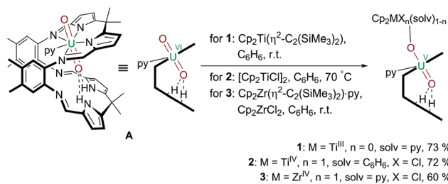
Scheme 1 Reductive metalation of A using Cp 2 Ti(η 2 -Me 3 -SiC≡CSiMe 3 ) ( 1 ), [Cp 2 TiCl] 2 ( 2 ), and Cp 2 ZrCl 2 /Cp 2 Zr(η 2 -Me 3 -SiC≡CSiMe 3 ) 2 ·py ( 3 ).
