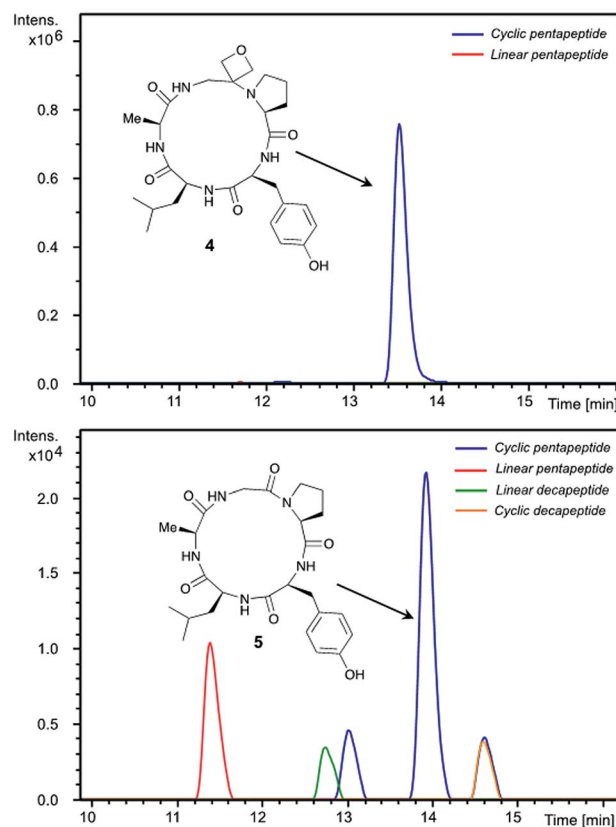
Fig. 1 Extracted ion chromatograms of peptide macrocyclisations [DEPBT (2 equiv.), ^1\text{Pr}_2\text{EtN} (2 equiv.), DMF (0.001 M), 48 h, RT] for 1 \rightarrow 4 (top) and 3 \rightarrow 5 (bottom).
