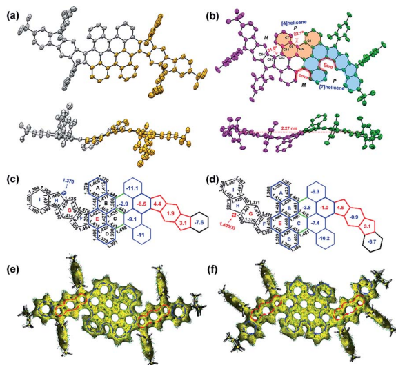
Fig. 3 Top view and side view of the X-ray crystallographic structure of (a) compound 1 (precursor for PH 1 ) and (b) tetraradicaloid 2 ; the hydrogen atoms are omitted for clarity. Selected bond lengths (Å) and calculated NICS(1) av values in the rings A–I of (c) 1 and (d) 2 . Calculated ACID plots of (e) 1 and (f) 2 . Isovalue is 0.05, and the blue and red arrows indicate diamagnetic and paramagnetic ring current flows, respectively.
