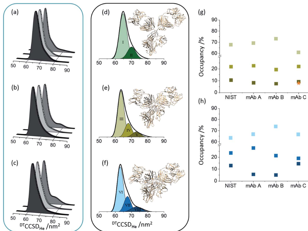
Fig. 2 Global collision cross section distributions ( DTCCSD_{He} ) for intact (a), endoS2 treated (b) and deglycosylated (c) Herceptin®; lot A (dark grey), lot B (light grey) and lot C (grey). Global CCSDs for intact (d), endoS2 treated (e) and deglycosylated (f) NIST mAb standard with fitted conformers. The darker the Gaussian for each sample, the more extended the conformer. The conformers present in each sample preparation have slightly different centres and FWHM values, hence different colours for each sample preparation. CCSDs for individual charge states for each sample and at each glycosylation level are provided in Fig. S7 in ESI.† Inserted mAb figures are snapshots from MD trajectories previously performed on pdb: 1IGY. 30 The image in (d) is from early in the MD simulation and therefore represents the intact mAb; later snapshots represent more contracted forms (e and f). Percentage occupancies of each conformer in the endoS2 treated samples (g) and deglycosylated samples (h) are presented with colours corresponding to the fitted Gaussians. For the endoS2 treated Herceptin® lot C there is an additional fourth extended Gaussian (see Fig. S6 in ESI†) which is represented by the orange star. Standard deviations between three day-to-day replicates are provided for the DTCCSD_{He} for individual charge states in Fig. S7 in ESI.†
