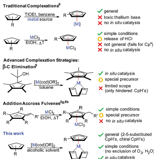
Fig. 1 Characteristics and drawbacks of complexation strategies for cyclopentadienyl ligands.
