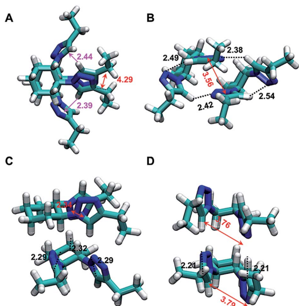
Fig. 10 Representation of the lowest free energy minima obtained in (A) a vacuum ( \otimes G = -1749.090117 au, BE = -19.33 kcal mol -1 ); (B) cyclohexane ( \otimes G = -1749.09237 au, BE = -16.35 kcal mol -1 ); (C) methanol ( \otimes G = -1749.106305 au, BE = -15.57 kcal mol -1 ); and (D) nitromethane ( \otimes G = -1749.106021 au, BE = -13.06 kcal mol -1 ). Hydrogen bonds are represented by dotted black lines, N-H \cdots \pi interactions as pink arrows and \pi - \pi stacking is shown as red double arrows. Labels refer to the distances (in Å) found for each stabilizing interaction: H \cdots O distance in the hydrogen bonds; H \cdots center of masses in N-H \cdots \pi interactions; and the center of masses to the center of masses in \pi - \pi stacking.
