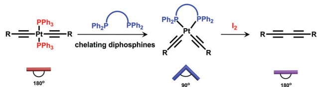
Scheme 1 Schematic representation of the successive transformations of the platinum-acetylide moiety with PPh 3 ligands.
