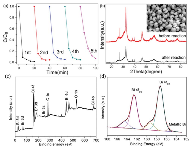
Fig. 7 (a) Reusability of Bi/OBr microflowers for photodegradation of TC; (b) XRD pattern and SEM result before and after 5 reusability tests; XPS spectra of the Bi/OBr after 5 reusability tests: (c) survey; (d) Bi 4f.
