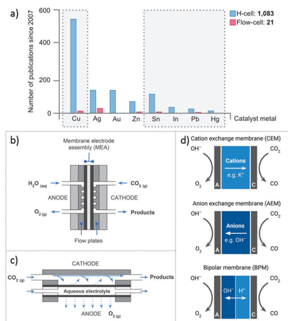
Fig. 24 (a) The number of papers published since 2007 on selected metal-based electrocatalysts for the \text{CO}_2\text{RR} in H-cells and in continuous flow reactors (data collected 29/12/2017). Cross-sectional diagrams of (b) a membrane-based reactor and (c) a microfluidic reactor. The former contains a membrane electrode assembly (MEA) consisting of the anode and cathode gas diffusion electrodes (GDEs) on either side of a polymer electrolyte membrane (PEM). In the schematized microfluidic reactor, the liquid electrolyte flows in the channel between the anode and cathode GDE materials, with \text{CO}_2 being supplied on the cathode side of the cell where it diffuses to the electrocatalyst supported on the cathode GDL. (d) Overview of different ion transport pathways between the anode and the cathode labeled "A" and "B", respectively, depending on the type of selected polymer electrolyte membrane. Readapted with permission from ref. 41. Copyright 2018 American Chemical Society.
