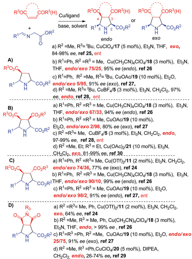
Scheme 6 exo -Selective cycloaddition of azomethine ylides with nitroalkenes catalyzed by Xing-Phos/Ag complex.
