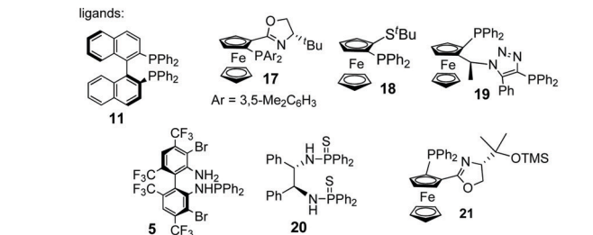
Scheme 8 Copper catalyzed 1,3-dipolar cycloaddition of azomethine ylides with \alpha,\beta -unsaturated carboxylic acid derivatives.
