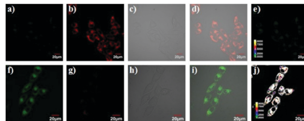
Fig. 76 Confocal fluorescence imaging without (up) and with (down) exogenous NaOCl (10 \mu\text{M} ) in MCF-7 cells using probe 51 (2 \mu\text{M} ) for 60 min at 37 ^\circ\text{C} ; (a and f) green channel (500–550 nm); (b and g) red channel (655–755 nm); (c and h) bright-field images; (d and i) overlay image of (a, b and c; f, g and h); (e and j) ratio images generated from green/red channel; \lambda_{\text{ex}} = 488 nm, 635 nm. Scale bar = 20 \mu\text{m} . Copyright 2017 Elsevier.
