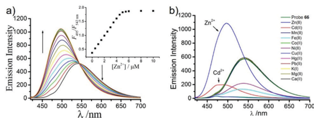
Fig. 110 (a) Fluorescence spectra of 5 \mu\text{M} 66 upon titration of Zn 2+ (0–10 \mu\text{M} ) in aqueous buffer (20 mM MES, 0.1 M NaCl, pH = 5.2), \lambda_{\text{ex}} = 405 \text{ nm} . Inset: The emission ratio ( F_{495}/F_{542\text{nm}} ) changes as a function of Zn 2+ concentration. (b) Fluorescence spectra of 66 ( 5 \mu\text{M} ) in the presence of various metal ions (5 \mu\text{M} Mn 2+ , Fe 2+ , Co 2+ , Ni 2+ , Cu 2+ , Zn 2+ , Cd 2+ , and 1 mM Mg 2+ , Ca 2+ , and K + ) in MES buffer (pH = 5.2, \lambda_{\text{ex}} = 405 \text{ nm} ). Copyright 2012 American Chemical Society.
