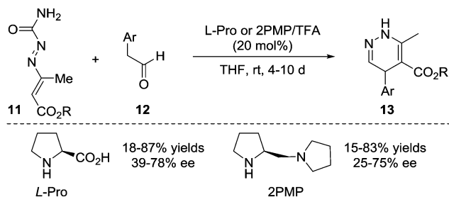
Scheme 6 Amine catalyzed formal [4+2] annulation of aldehydes with azoalkenes.
