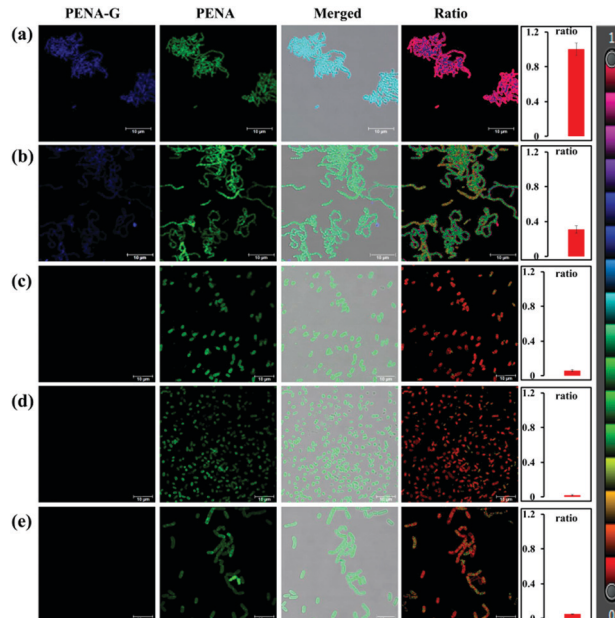
Fig. 2 Fluorescence images of various bacteria in the presence of PENA (50 \mu\text{M} ). (a) Streptococcus mutans ; (b) Hemolytic streptococcus ; (c) Lactobacillus amylovorus (d) Streptococcus pasteurianus strain 080205; (e) Bacillus cereus 994000168 LBK. Fluorescence ratio ( I_{415-465}/I_{535-585} nm), PENA-G \lambda_{\text{ex}} 405/ \lambda_{\text{em}} 415–465 nm, PENA \lambda_{\text{ex}} 405/ \lambda_{\text{em}} 535–585 nm, Scale bar 10 \mu\text{m} .
