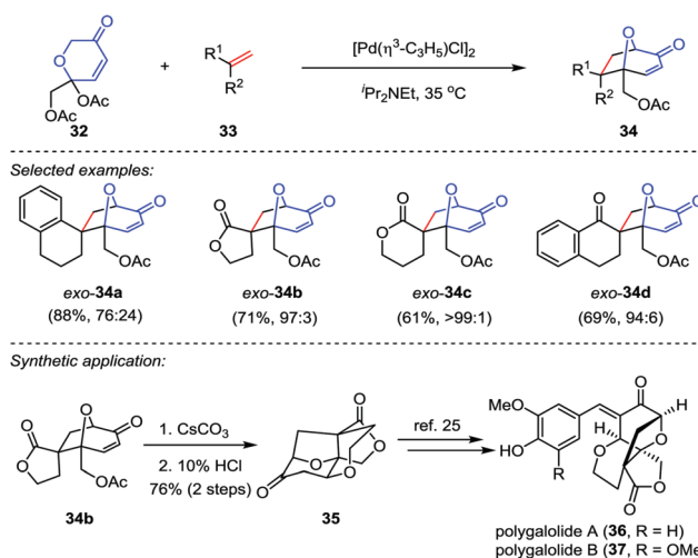
Scheme 7 The [\text{Pd}(\eta^3\text{-C}_3\text{H}_5)\text{Cl}]_2 -catalyzed [5+2] cycloaddition by Suga and co-workers.
