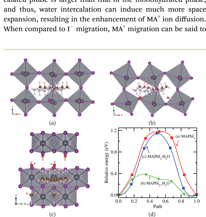
Fig. 5 \text{MA}^+ ion migration in (a) pseudo-cubic \text{MAPbI}_3 , (b) water intercalated phase \text{MAPbI}_3 \cdot \text{H}_2\text{O} and (c) monohydrated phase \text{MAPbI}_3 \cdot \text{H}_2\text{O} , and (d) corresponding activation energy profile.
