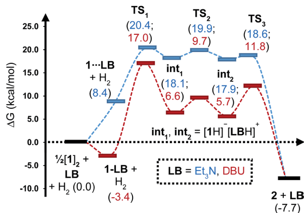
Fig. 5 Computed free energy profile for Et 3 N- and DBU-assisted H 2 activation with 1 . Relative free energies (in kcal mol -1 ) are with respect to 0.5[\text{1}]_2 + \text{LB} + \text{H}_2 .
