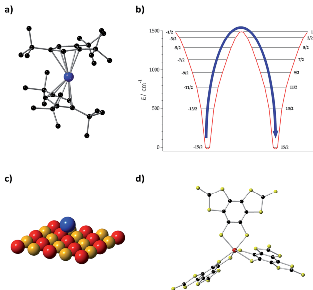
Fig. 5 (a) Molecular structure of [\text{Dy}(\text{Cp}^{\text{ttr}})_2]^+ , where \text{Cp}^{\text{ttr}} = \{\text{C}_5\text{H}_2^t\text{Bu}_3\text{-}1,2,4\} and ^t\text{Bu} = \text{C}(\text{CH}_3)_3 . H atoms are omitted for clarity. Dy: blue and C: black. (b) Energy levels and M_J projections of [\text{Dy}(\text{Cp}^{\text{ttr}})_2]^+ , determined by CASSCF-SO calculations. (c) Ho atom on a MgO monolayer. Mg: yellow and O: red. (d) Molecular structure of [\text{V}(\text{C}_8\text{S}_8)_3]^{2-} . V: red, C: black, and S: yellow.
