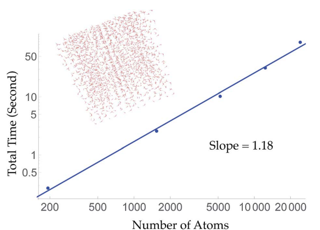
Fig. 2 Aperiodic timings of an energy, charge and force call for cubic water clusters at a density of 1 g cm -3 . The largest \sim 60 Angstrom cube is 4 \times larger than the electrostatic cutoff. The slope of a log–log version of this curve is near unity, indicating the wall-time scaling of TensorMol. Inset figure: the cubic water cluster used for timing containing 1728 water molecules.
