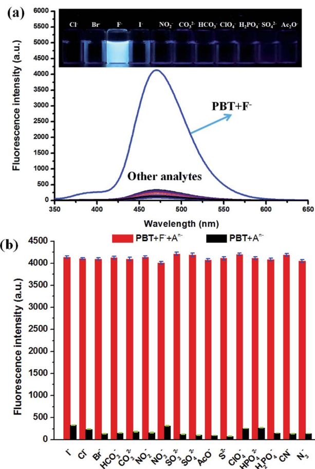
Fig. 6 (a) Fluorescence spectra of PBT in the presence of various anions. [PBT] = 10 \mu\text{M} , [An^-] = 20 \mu\text{M} , in a mixture of THF and Tris buffer solution ( \text{pH } 8.0 ), (1 : 9, v/v), \lambda_{\text{ex}} = 335 \text{ nm} , \lambda_{\text{em}} = 470 \text{ nm} . Inset: direct observation of fluorescence emission difference of the probe PBT ( 10 \mu\text{M} ) under UV irradiation ( 365 \text{ nm} ) in the presence of different anions. Left to right: \text{Cl}^- , \text{Br}^- , \text{I}^- , \text{F}^- , \text{NO}_2^- , \text{CO}_3^{2-} , \text{HCO}_3^- , \text{ClO}_4^- , \text{H}_2\text{PO}_4^- , \text{SO}_4^{2-} and \text{AcO}^- . (b) The selectivity of PBT in the presence of various anions.
