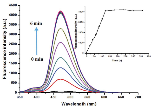
Fig. 5 Time course of the signaling of PBT by F^- [PBT is 10 \mu\text{M} , [F^-] is 20 \mu\text{M} ], in a mixture of THF and Tris buffer solution ( \text{pH } 8.0 ), (1 : 9, v/v), \lambda_{\text{ex}} = 335 \text{ nm} , \lambda_{\text{em}} = 470 \text{ nm} . Inset: the response curve of fluorescence intensity of PBT with F^- depending on the various time.
