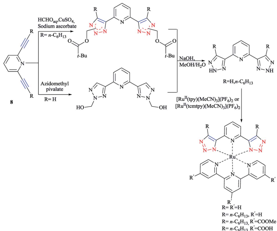
Scheme 7 Synthesis of bis(tridentate)ruthenium(II) complexes.
