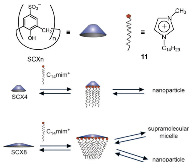
Fig. 9 Schematic representation of different self-assemblies formed by different p -sulfonatocalix[ n ]arenes (SCX n , n = 4 or 8 ). Adapted with permission from ref. 53. Copyright 2017 American Chemical Society.
