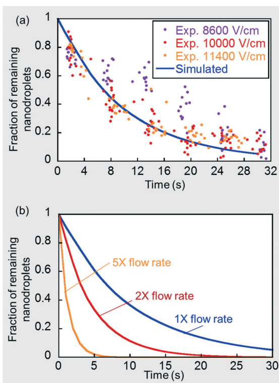
Fig. 7 (a) Simulation of the convection-controlled scenario and comparison to experimental results under a CP flow rate of 50 μL min -1 and DP flow rate of 10 μL min -1 . (b) Convection-controlled simulation results at 5×, 2×, and 1× of the base flow rate of 50 μL min -1 (CP) and 10 μL min -1 (DP).
