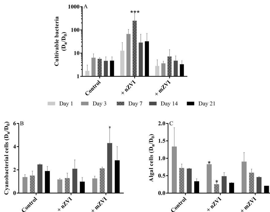
Fig. 4 Abundance of planktonic microorganisms (fold change of D_n/D_0 over the 21 day experiment using reservoir water with nZVI (+ nZVI), reservoir water with mZVI (+ mZVI), and reservoir water only as a control); (A) cultivable bacteria, (B) cyanobacterial number and (C) green algae number. Note: different scales for the y axis. Error bars n = 3 . Statistically significant differences (* P < 0.05 , ** P < 0.01 and *** P < 0.001 ) compare the treatment to the control. The actual number of cells is provided in the ESI† (Table S2).
