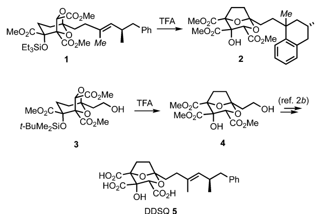
Scheme 1 Transketalisation approaches to (–)-6,7-dideoxysqualstatin H5.
