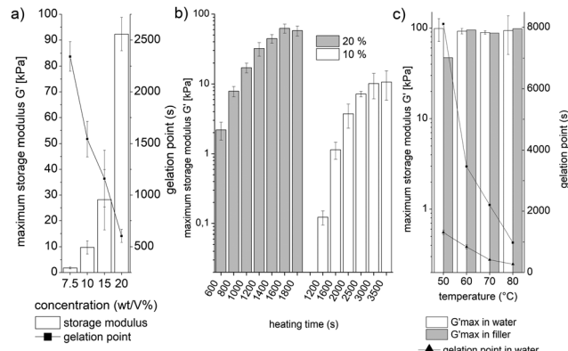
Fig. 2 Hydrogel characterization (maximum G' and gelation point) (procedures and detailed conditions are listed in the ESI † ). (a) Variation of sPEG concentration for heating at 60 °C, (b) the effect of different heating times at 60 °C for both 10 and 20 wt/V%, (c) gelation at different temperatures for both water and non-volatile PEG filler as a dispersing agent (20 wt/V% reactive sPEG); measurements are reproduced three times except for 2c with the filler due to long gelation times.
