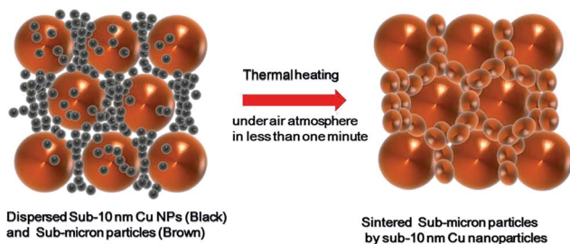
Fig. 30 Schematic illustration of the sintering mechanism of the copper-based composite inks. [Reprinted with permission from ref. 269 Copyright \text{©} American Chemical Society.]
