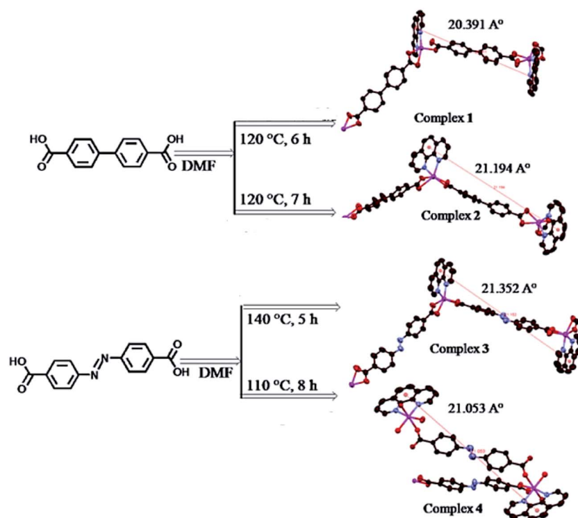
Scheme 14 CPs obtained by the reaction of metal [Zn(\text{II}), \text{Cd}(\text{II})] , phen separately with biphenyl-4,4'-dicarboxylic acid and 4,4'-azodibenzoic acid. [Reprinted with permission from ref. 170. Copyright 2012, American Chemical Society.]
