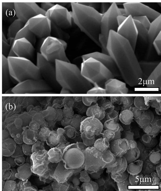
Fig. 32 SEM images of thermal decomposition residue of [\text{ZnCl}_2\text{L}] (a) and [\text{ZnBr}_2\text{L}] (b) calcined at 500^\circ\text{C} for 2 h. [Reproduced from ref. 320 with permission from The Royal Society of Chemistry.]
