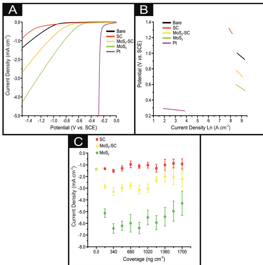
Fig. 2 (A) Linear sweep voltammetry (LSV) of bare/unmodified SPE, SPE modified with ca. 2.8 mg cm -2 of SC, SPE modified with ca. 1725 ng cm -2 of 2D-MoS 2 , SPE modified with ca. 1725 ng cm -2 of 2D-MoS 2 -SC and a Pt electrode showing the onset of the HER. Scan rate; 250 mV s -1 (vs. SCE). Solution composition: 0.5 M H 2 SO 4 . (B) Tafel analysis; potential vs. Ln of current density for faradaic section of the LSV presented in (A). (C) The current densities observed at -1.5 V for SPEs modified with 172, 345, 518, 690, 863, 1035, 1207, 1380, 1553 and 1726 ng cm -2 of 2D-MoS 2 (green circles) and 2D-MoS 2 -SC (yellow triangles) as well as SPEs modified with ca. 282, 565, 848, 1131, 1414, 1697, 1980, 2263, 2545, 2828 mg cm -2 of SC (red squares) (average standard deviation of 3 replicates). Scan rate; 250 mV s -1 (vs. SCE). Solution composition: 0.5 M H 2 SO 4 .
