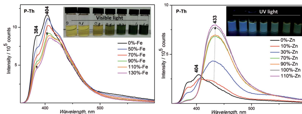
Fig. 5 Emission spectra of P-Th with increasing amounts of Zn^{2+} and Fe^{2+} metal ions. Inset: captured pictures of samples, Zn^{2+} -UV light, Fe^{2+} -visible light.
