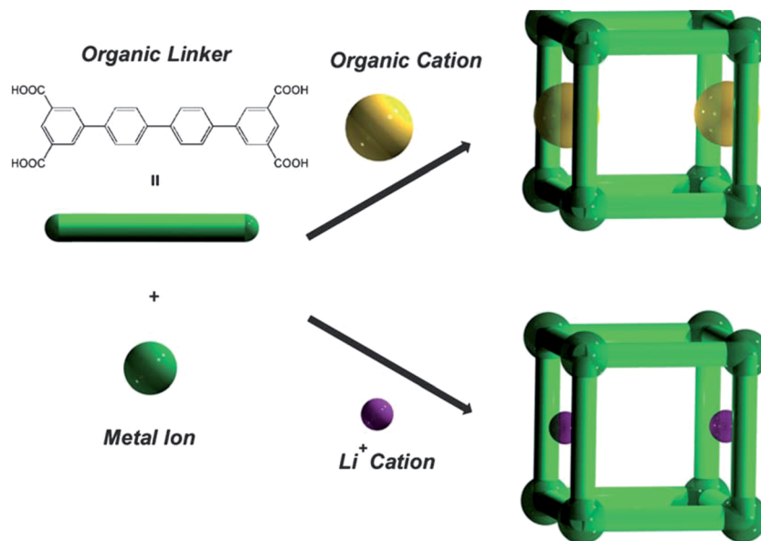
Fig. 14 A schematic representation of the construction of modulated MOFs in \{(\text{A})[\text{In}(\text{L}^7)]\cdot\text{solv}\}_\infty (69) with different pore gates. Reproduced with permission from ref. 109, copyright 2011, Royal Society of Chemistry.
