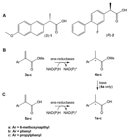
Scheme 1 (A) Profens: ( S )-naproxen 1a , ( R )-flurbiprofen 2 . (B) and (C) Proposed ene-reductase-catalysed steps in the chemoenzymatic synthesis of profens.
