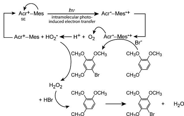
Fig. 12 Schematic representation of the photocatalytic bromination of 1,2,4-trimethoxybenzene (TMB) with 9-mesityl-10-methylacridinium ( \text{Acr}^+-\text{Mes} ) as a catalyst. SE: Singlet excited state.
