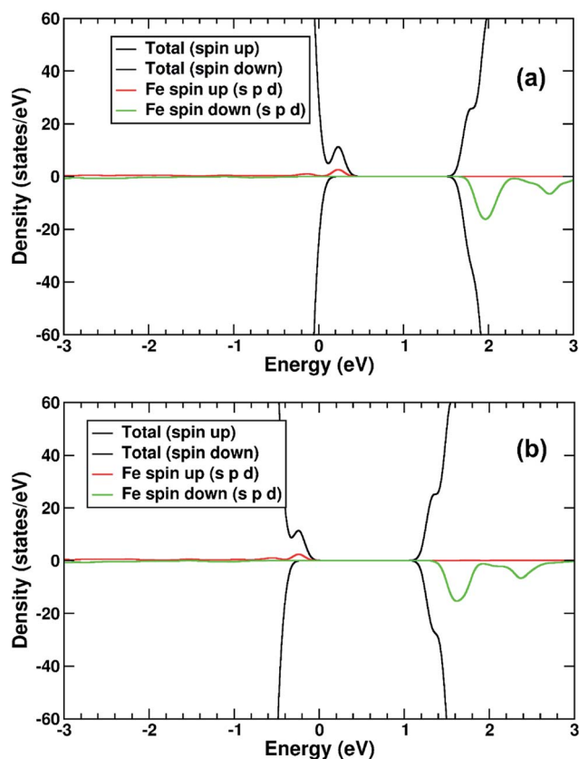
Fig. 8 (a) DOS of \text{TiO}_2(R)\text{-Fe(V}_{\text{Ti}}) . (b) DOS of the electronic polaron structure of \text{TiO}_2(R)\text{-Fe(V}_{\text{Ti}}) . The red line represents projection of Fe states in spin up channel, green line projection of Fe states in spin down channel. The zero of the x-axis is set to the top of the VBM.
