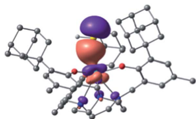
Fig. 6 Bonding \sigma orbital of [[(\text{Ad,MeArO})_3\text{tacn}]\text{U-SH}] (2).
