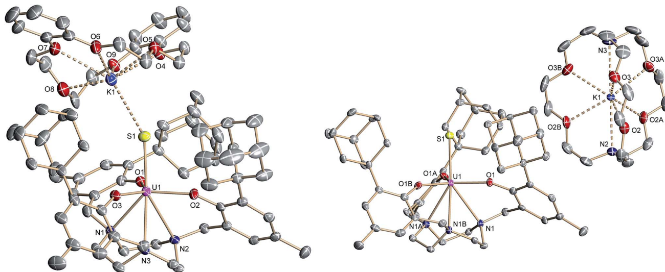
Fig. 2 Molecular structure of the uranium(IV) sulfido complex [(^{\text{Ad,Me}}\text{ArO})_3\text{tacn)U}\equiv\text{S}\cdots\text{K}(\text{db-18-c-6}) ( 3 ) (left), and [(^{\text{Ad,Me}}\text{ArO})_3\text{tacn)U}\equiv\text{S}] ( 4 ) (right). All hydrogen atoms and the solvent molecules are omitted for clarity (50% probability ellipsoids).
