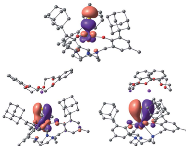
Fig. 7 U–S bonding orbitals in [[(\text{Ad,MeArO})_3\text{tacn}]\text{U}\equiv\text{S}\cdots\text{K}(\text{db-18-c-6})] (3), with the \sigma (top) and the set of two \pi orbitals (bottom).
