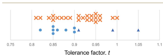
Fig. 1 The tolerance factors of \text{ABI}_3 compounds. Blue dots represent inorganic \text{ABI}_3 compounds that form perovskites at room temperature and pressure. Red crosses represent inorganic \text{ABI}_3 compounds that do not form perovskites. Blue triangles show hybrid \text{APbI}_3 and \text{ASnI}_3 compounds that form in the perovskite structure, using the methodology of Cheetham et al. to estimate molecular ion radii. 26,27 There is no boundary on the tolerance factor scale that separates perovskites from non-perovskites.
