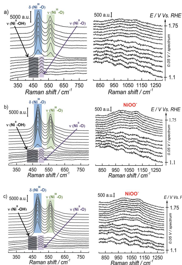
Fig. 2 SER spectra obtained at constant potential during the electrochemical oxidation of Ni(OH) 2 and the subsequent OER on NiOOH at different pH's. The ionic strength of the solution was fixed to 0.1 M with NaClO 4 except for pH 13, that solution is NaOH 0.1 M. The left panel presents the spectra in the wavenumber region 300–800 cm -1 and the right panel presents the wavenumber region 800–1300 cm -1 : (a) pH 11, (b) pH 12.0, (c) pH 13.0.
