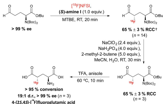
Scheme 7 Organomediated radiosynthesis of ^{18}\text{F} -(2 S ,4 S )-4-F-LGU. \dagger RCC determined by radio-HPLC relative to ^{18}\text{F} -NFSI.
