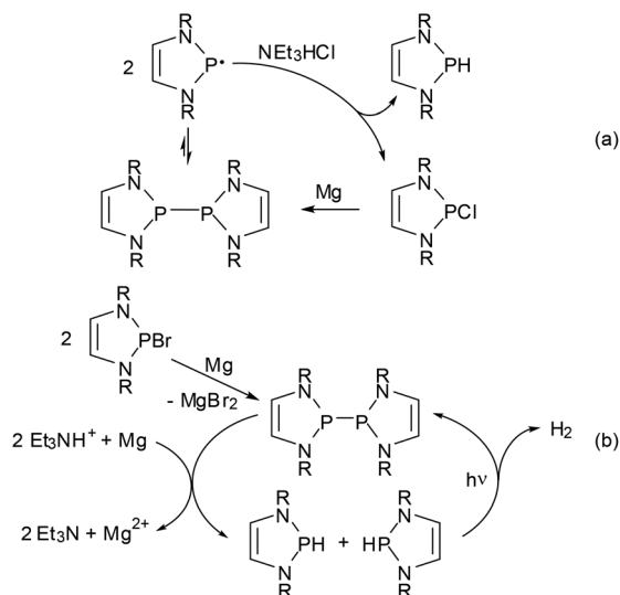
Scheme 14 (a) Reduction of Cl-DAPs to H-DAPs using Mg/Et 3 NHCl via disproportionation of diazaphospholenyl radicals as the key step (R = Dipp, 2- t BuC 6 H 4 ); 15 (b) photocatalytic reductive generation of H 2 (R = Dipp). 61 Both reactions can also be performed with CC-saturated NHPs. Generation of the bis-diazaphospholenyl in (b) can be performed in situ from a Br-NHP precursor.
