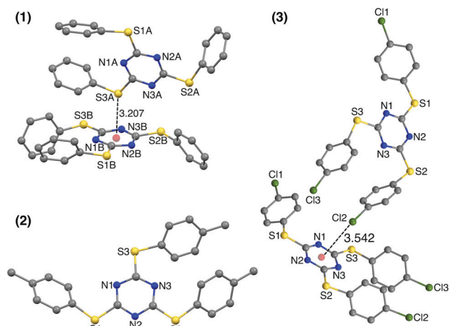
Fig. 1 X-ray structures of 2,4,6-tris(phenylthio)-1,3,5-triazine (1), 2,4,6-tris( p -tolylthio)-1,3,5-triazine (2), and 2,4,6-tris((4-chlorophenyl)thio)-1,3,5-triazine (3). The hydrogen atoms are not shown for clarity. Intramolecular \pi\cdots\pi interactions: (1) 4.287 and 4.350; (2) 4.384; (3) 4.158 Å.
