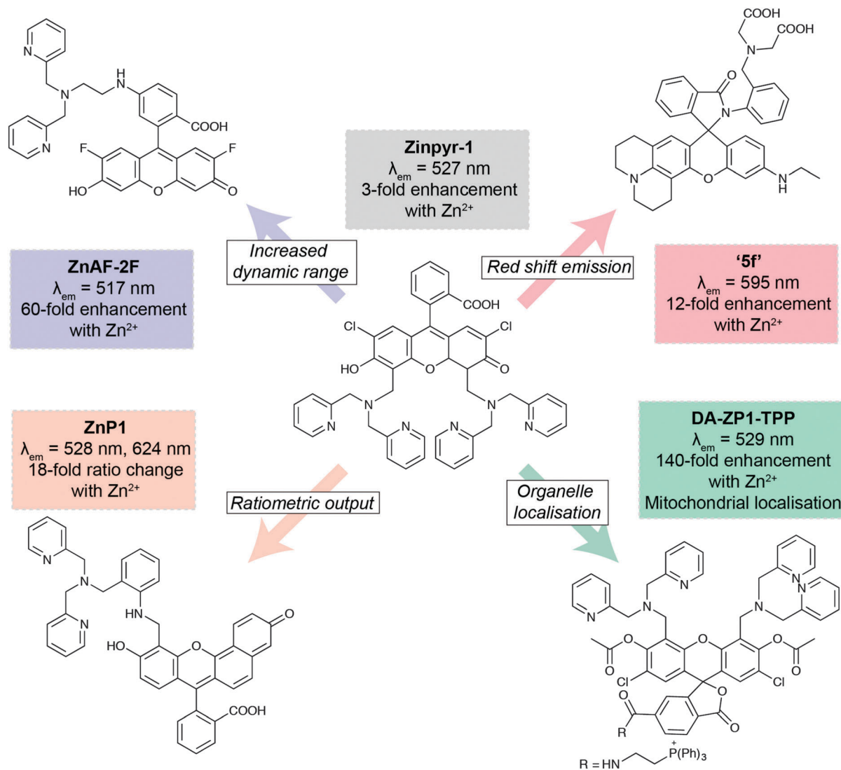
Fig. 6 Key developments in xanthenone-based fluorescent sensors for \text{Zn}^{2+} . Zinpyr-1 98 has been further developed to improve the range of \text{Zn}^{2+} concentrations it can detect ( ZnAF-2F ), 99 measure \text{Zn}^{2+} flux via ratiometric measurements ( ZnP1 ), 100 localise within specific organelles, such as mitochondria ( DA-ZP1-TPP ), 101 and optimise its fluorescence emission peak ( 5f ). 102
