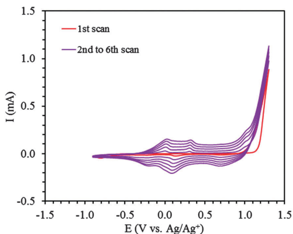
Fig. 3 Electrochemical polymerization of ProDOT-diene ( 5 \text{mM} ) in ACN-TBAP ( 0.1 M). 1st scan (red), subsequent scans, 2nd to 6th (purple).
